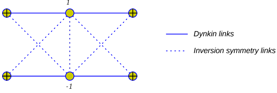
Figure 3: The Dynkin diagram for the PSU(1, 1|2) \times PSU(1, 1|2)/SU(1, 1) \times SU(2) coset.
