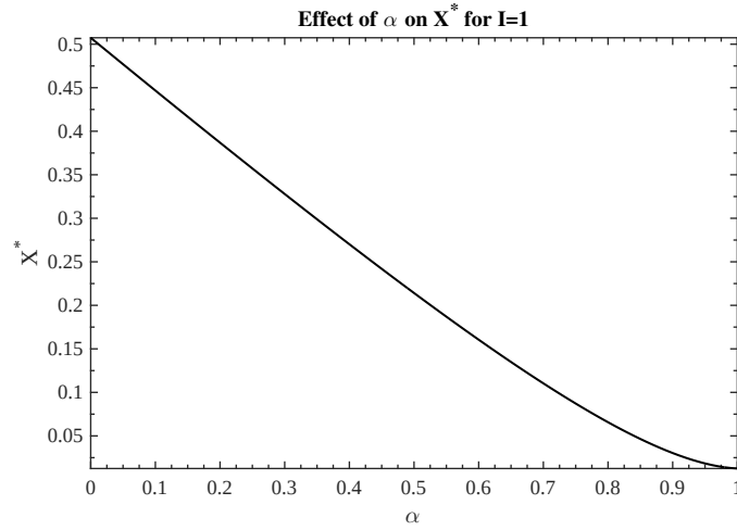
Figure 1: Parameter values: I = 1 , \phi = 0.5 , \lambda = 0.5 , \kappa(\alpha) := 1 - 0.75\alpha , \sigma = 0.2 , r = 0.05 , \mu = 0.02 .
