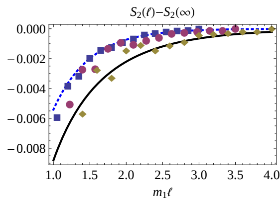
Figure 6: The function (51) (solid curve), compared to TCSA results obtained in [7] for a system of length m_1L = 8 (rombi), m_1L = 7 (circles) and m_1L = 6 (squares) and to the fit (60) (dashed curve).
