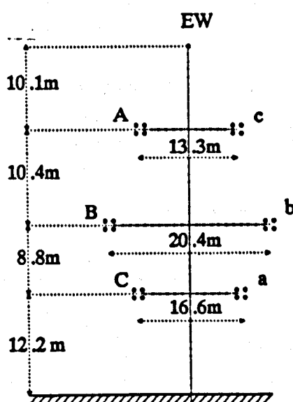
Fig. 5-3 Double-circuit line
