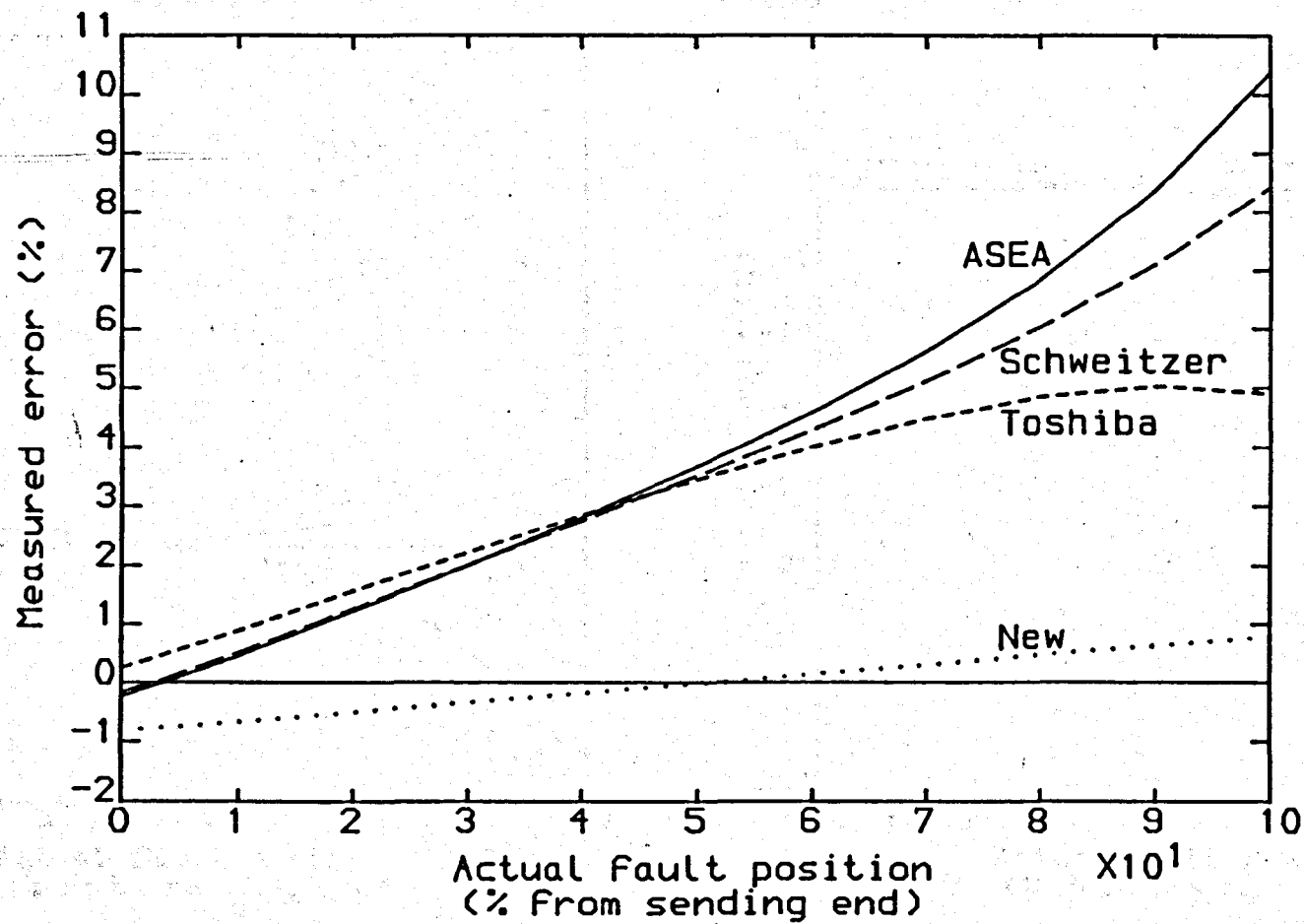
Fig. 7-4 Effect of [Z] matrix errors on the locators' accuracy for an utransposed line
