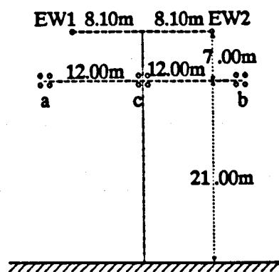
Fig. 5-1 Horizontal single-circuit line
