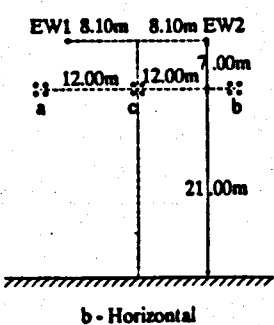
Fig. 3 Line configurations
