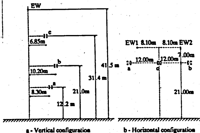
Fig. 3- Line configurations
