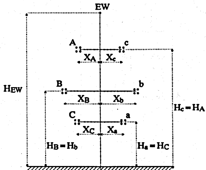
Fig. 3-1 Double-circuit line vertical configuration
