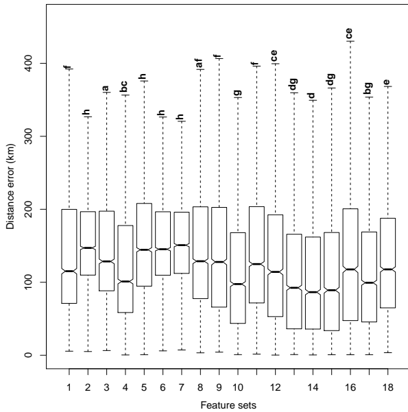
Figure 3: Distance error of predictions for different sets of features (see Table 3 for the feature set used to train each model). Labels a-l indicate features sets that have non-significantly different results ( p > \hat{\alpha} ) where they share the same letter. For example, feature set 3 shares the label a with feature set 8 but shares no label with any other feature set, indicating that results from model 3 are significantly different from all other models except for model 8.
