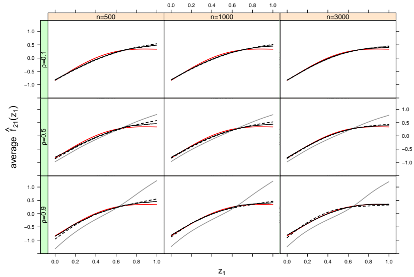
FIG 5. Average fits calculated using the estimated smooth functions for \hat{f}_{21}(z_1) based on 1000 replications when employing the naive (grey solid lines), multiple-stage (black dashed lines) and bivariate probit (black solid lines) estimation approaches. The true function is represented by the red solid lines. Note that in some cases the curves differ only minimally, hence they can hardly be distinguished. Further details are given in the caption of Figure 2.
