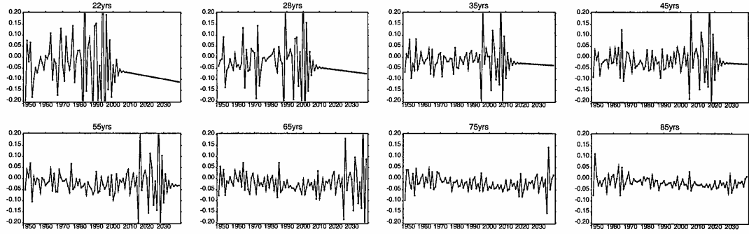
(b) UK male assured lives study: model H(1)
