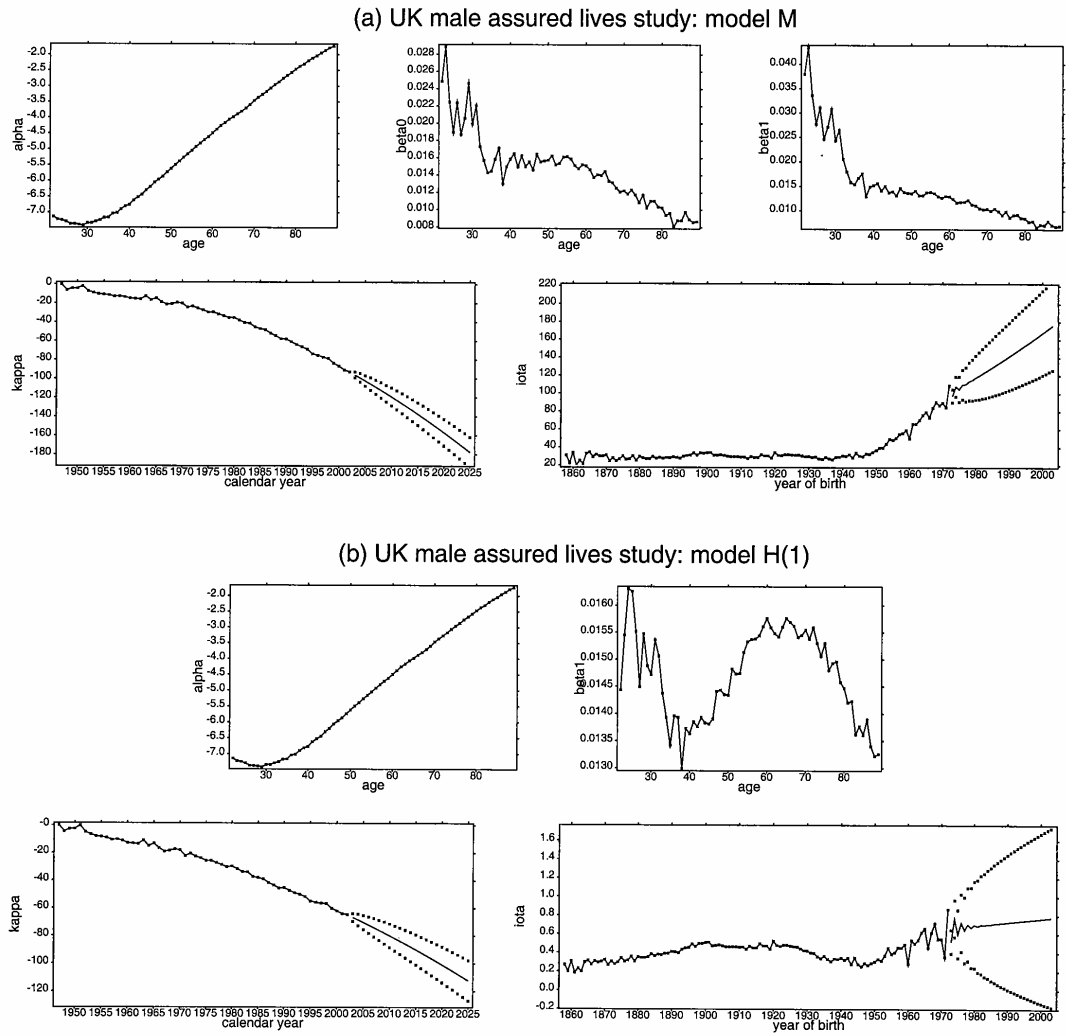
Fig. 5. UK male assured lives study, parameter estimates- (a) model M; (b) model H 1
