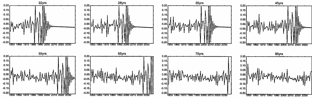
Fig. 9. Secular trends in \frac{1}{\mu_{xt}} \frac{\partial \mu_{xt}}{\partial t} for selected ages x , UK male assured lives study, incorporating- (a) model M projections; (b) model H 1 projections
