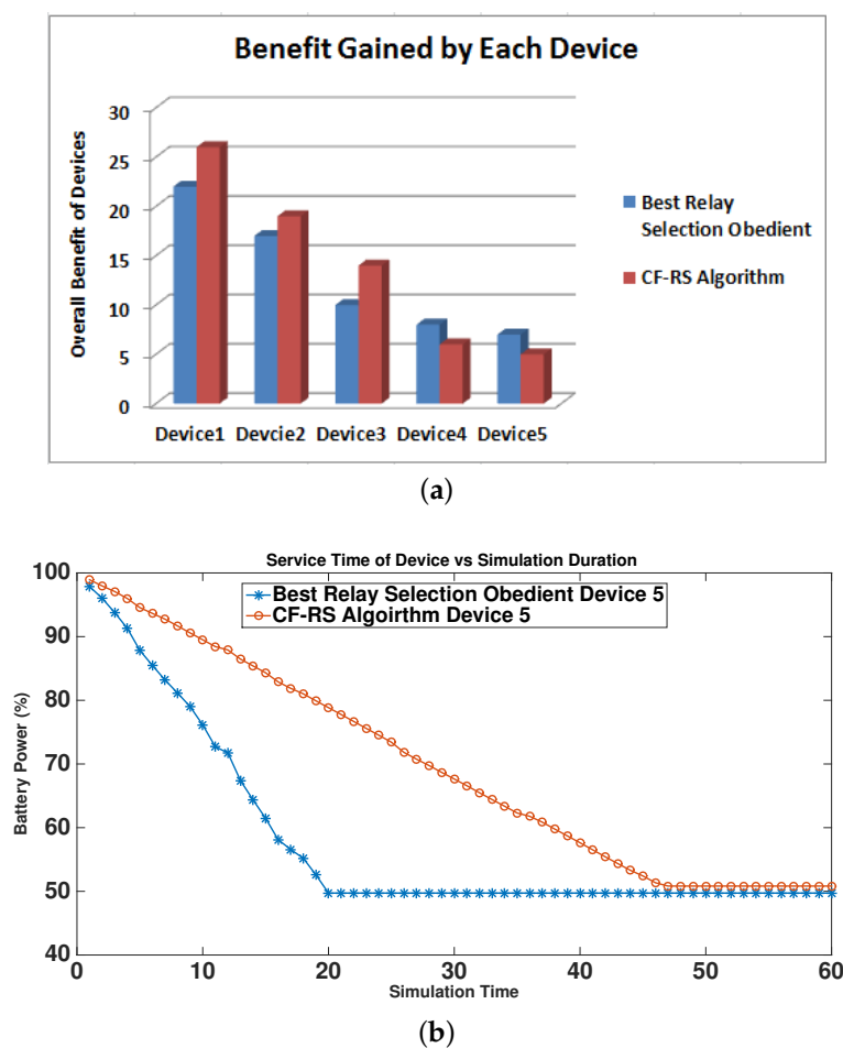
Figure 8. Variation 1: best relay selection with obedient relays: (a) overall benefit attained by devices; (b) service time of D5 .
