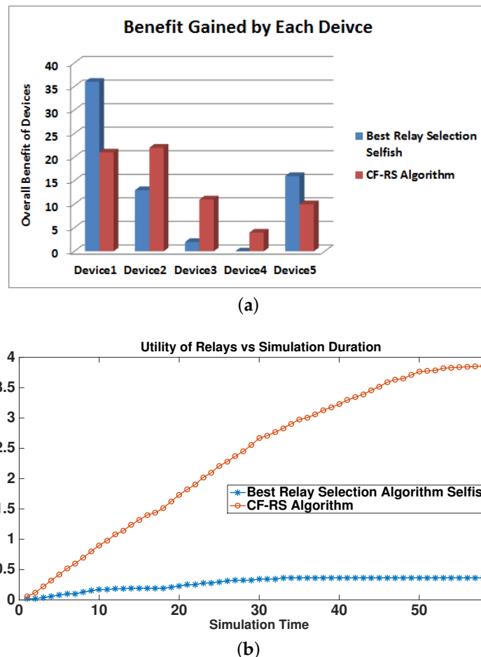
Figure 11. (a) Overall benefit attained by devices for the test case Scenario 2 where the relays and end devices swapped their positions multiple times and (b) the cumulative utility of devices D1 , D2 , D3 , D4 and D5 for the test case Scenario 2 when acting as relays.
