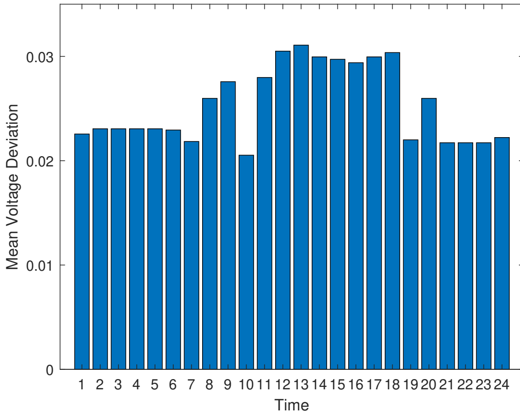
Fig. 3.9 Average Voltage deviation from the reference voltage for 24 hours
