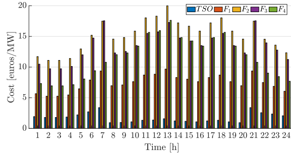
Fig. 5.16 TSO and DSOs operational cost using the proposed centralised coordination scheme.
