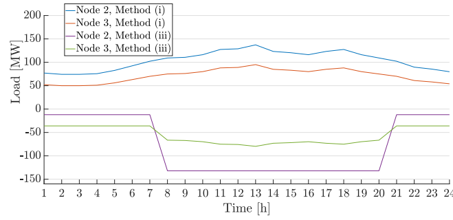
Fig. 5.15 Net load at nodes 2,3 with using methods (i) and (iii).
