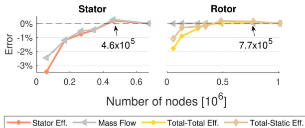
Fig. 5 Grid independence study for rotor and stator
