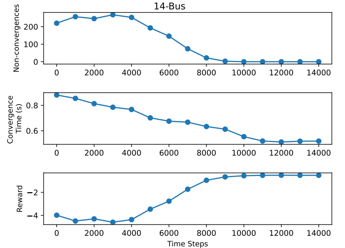
Figure 2. PPO-GNN training statistics for 14-bus test case. The three scatter plots represent the number of non-convergences, average IPS convergence time, and average reward on the y-axis and the number of time steps on the x-axis.
