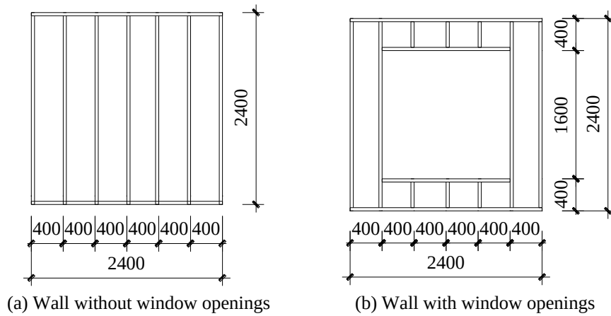
Fig. 2. Elevation of the wall (mm).
