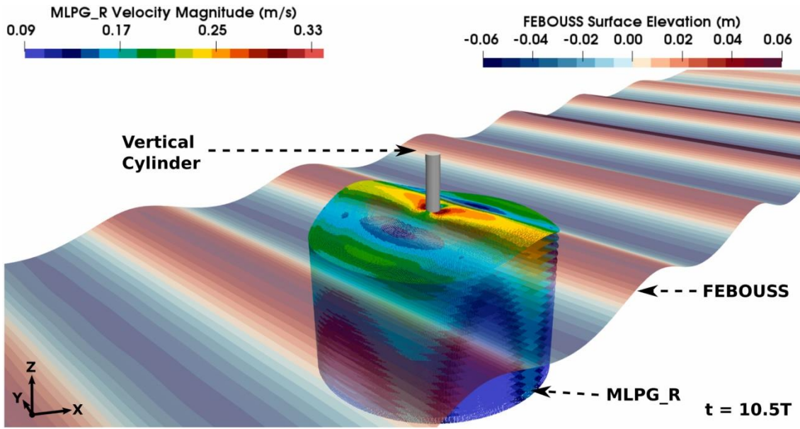
Figure 8. Simulation of directional regular waves (aligned at 30^\circ to the x -axis) interacting with a fixed cylinder using weakly coupled FEBUOUS and MLPG_R using 3D cylindrical coupling interfaces (Agarwal et al., 2022b).
