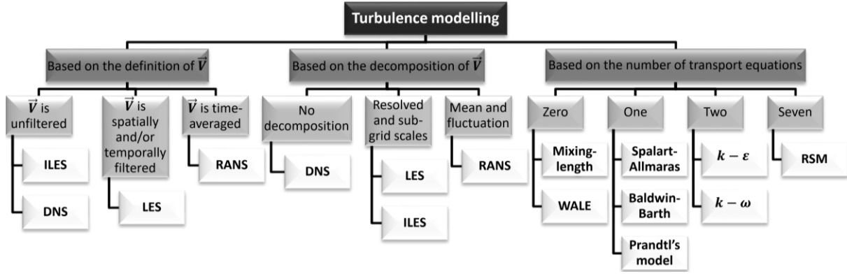
Figure 4. An illustration of the different means to categorize various strategies to model turbulence in depth-resolving models; cf. nomenclature for the abbreviations.
