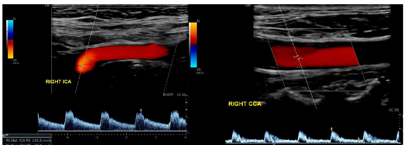
Fig. 2. Sonograms of the right internal (ICA) and common carotid arteries (CCA) showing spectral Doppler waveforms and measurements of the PSV and EDV within the lumen of the vessels – images by E.A.
