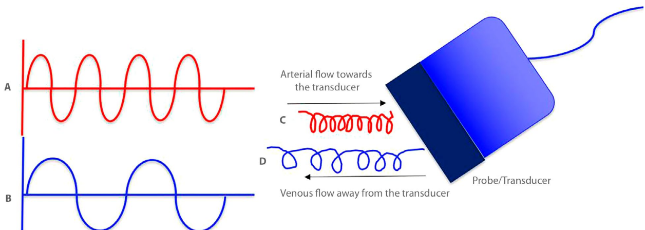
Fig. 1. Waveforms of arterial blood (A) flow towards the transducer, and venous blood (B) flow away from the transducer. The waveforms illustrate a higher frequency (4 cycles per second) of the arterial flow (a positive shift) than the venous flow frequency (2 cycles per second) within the same period. This is further illustrated (C, D) using metal spring diagrams where there are more compressions on the spring pattern representing flow towards the transducer and more regions of rarefactions on the spring pattern representing flow away from the transducer
