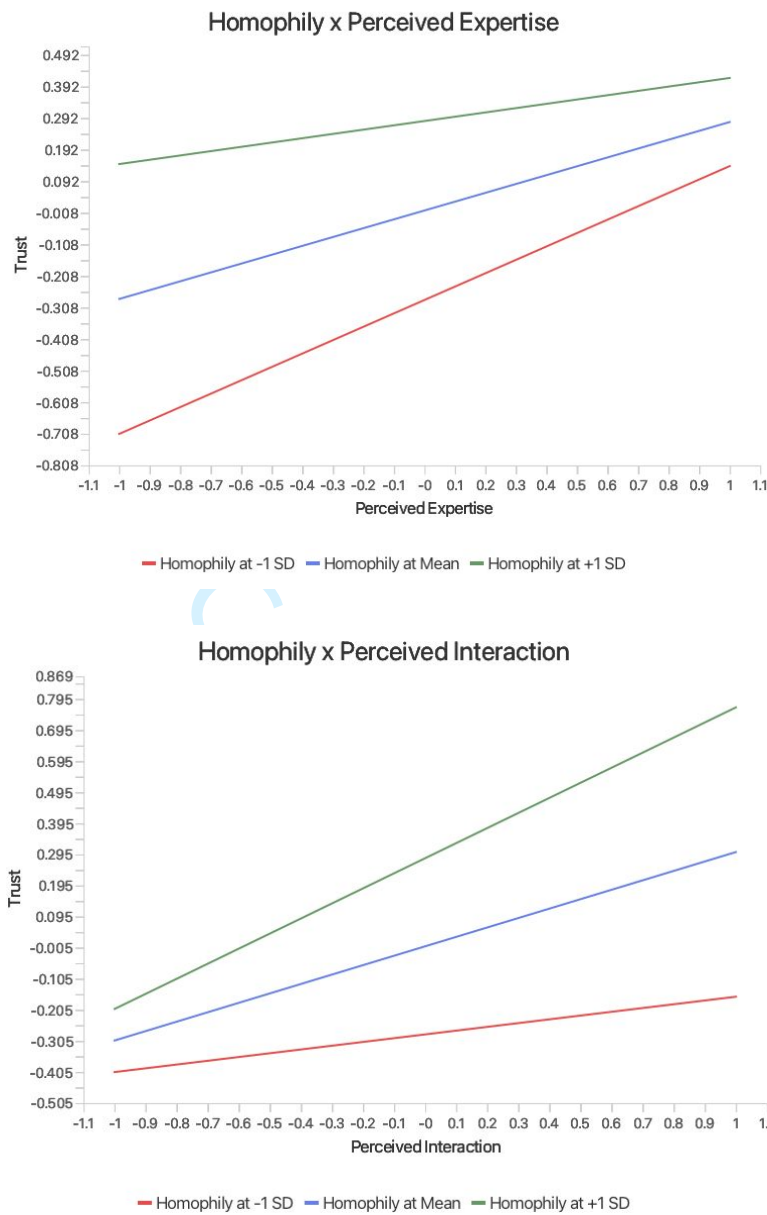
Fig. 3. Simple slope analysis
