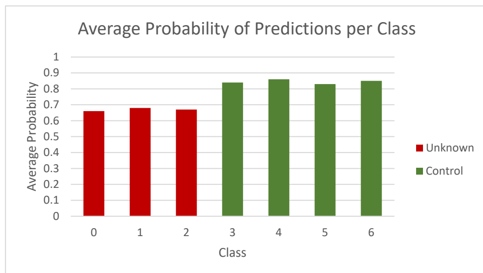
Figure 9. Average probabilities for known (green) and unknown (red) classes, for CIFAR-10 experiment.
