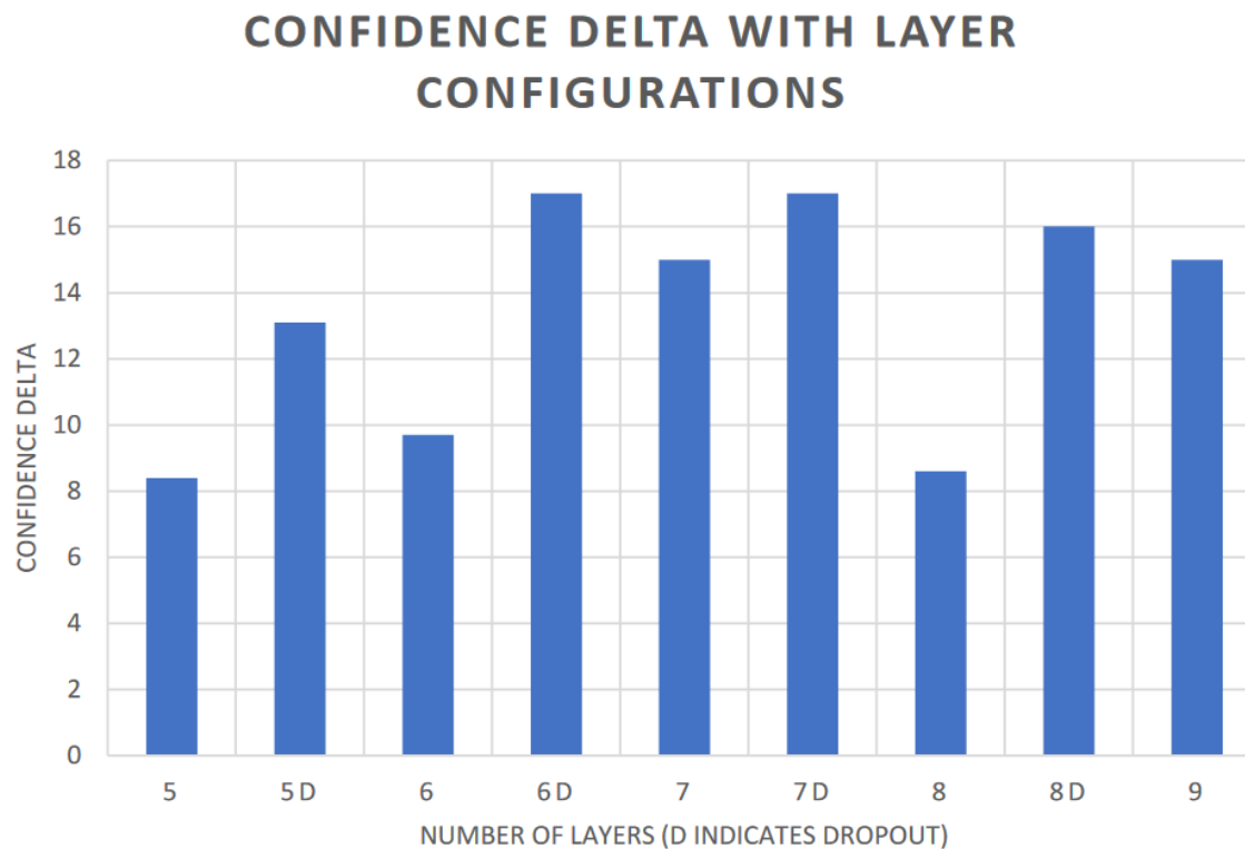
Figure 5. Effect of layers and dropout on confidence delta.
