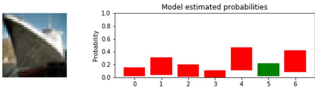
Figure 11. Distributed label probabilities for unknown image (ship). Here, the green bar represents a false positive from relabelling, with the red bars indicating incorrect classification.
