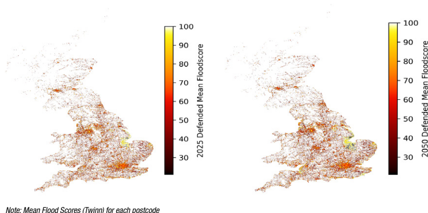
FIGURE 1: FLOOD RISKS IN BRITAIN IN 2025 AND 2050 3
