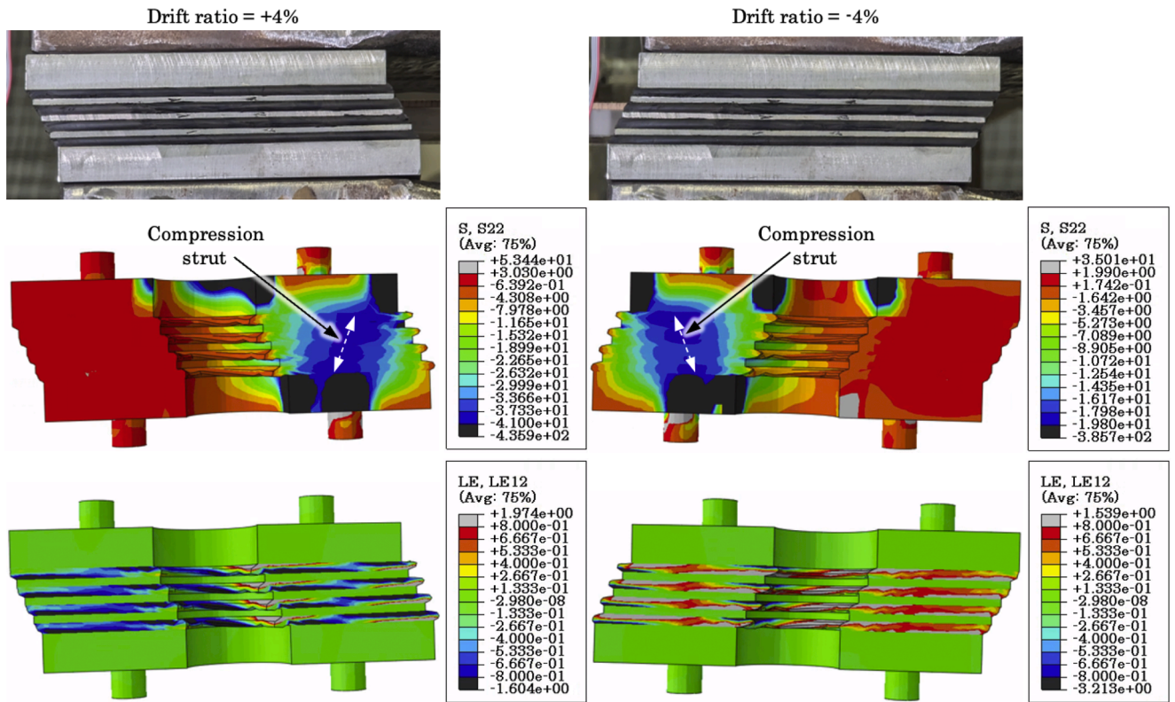
Fig. 18. Deformation, stress, and strain distribution in the rubber bearings.
