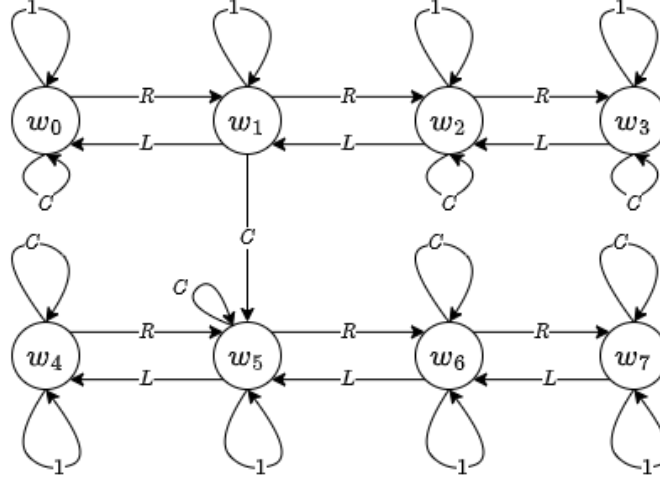
Figure 11: Minimum action network for world \mathcal{W}_{consumable} .
