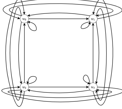
Figure 2: A transition diagram for the transitions shown in Table 1.
