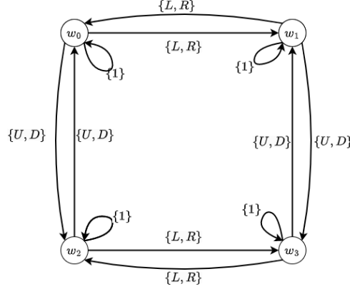
Figure 5: Action equivalence classes in A/\sim for the actions show in Figure 3.
