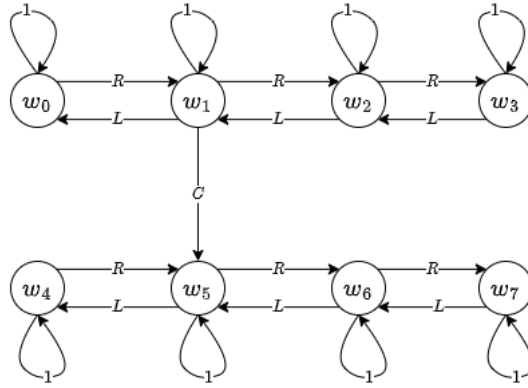
Figure 13: Minimum action network for a world containing an agent and a consumable.
