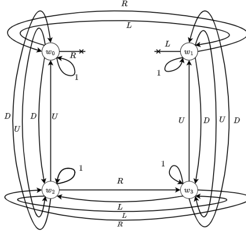
Figure 12: A diagram of the labelled transitions in Table 13.
