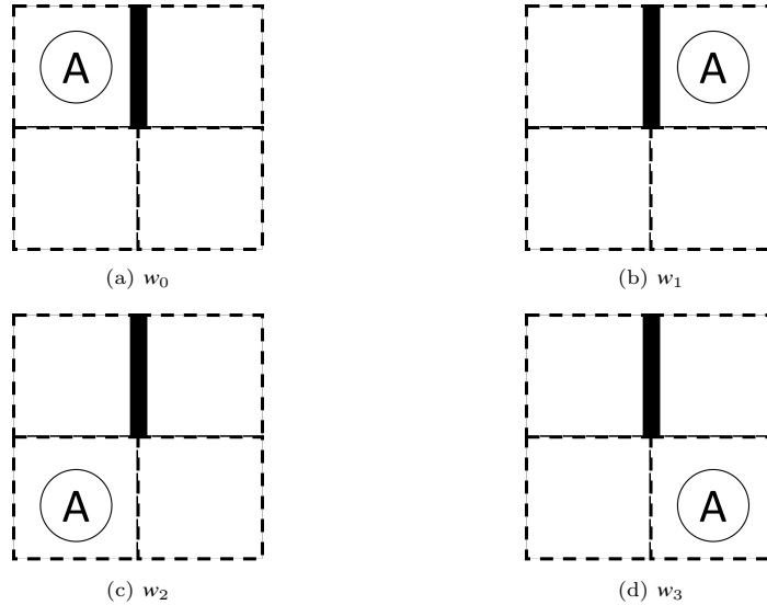
Figure 6: The world states of a cyclical 2 \times 2 grid world \mathcal{W}_{wall} with a wall, where changes to the world are due to an agent moving either up, down, left, or right. The position of the agent in the world is represented by the position of the circled A. The treatment of the wall is explained when needed.
