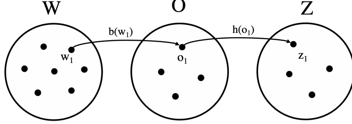
Figure 4: The composite mapping from the set W of world states to the set Z of state representations via the set O of observations.
