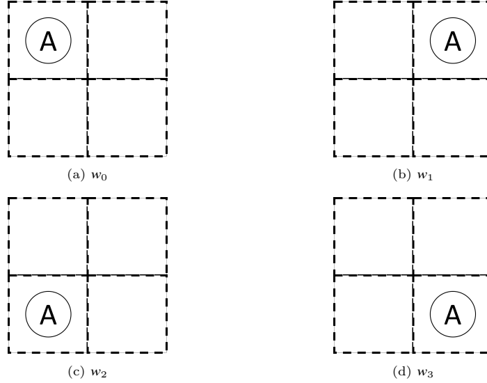
Figure 1: The world states of a cyclical 2 \times 2 grid world W_c , where changes to the world are due to an agent moving either up, down, left, or right. The position of the agent in the world is represented by the position of the circled A.
