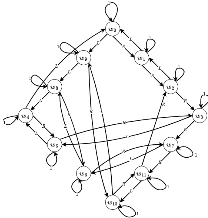
Figure 9: A transition diagram of the labelled transitions in Table 10.
