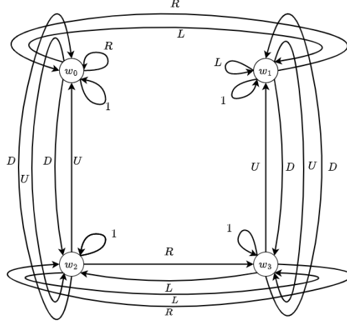
Figure 7: A transition diagram of the labelled transitions in Table 8.
