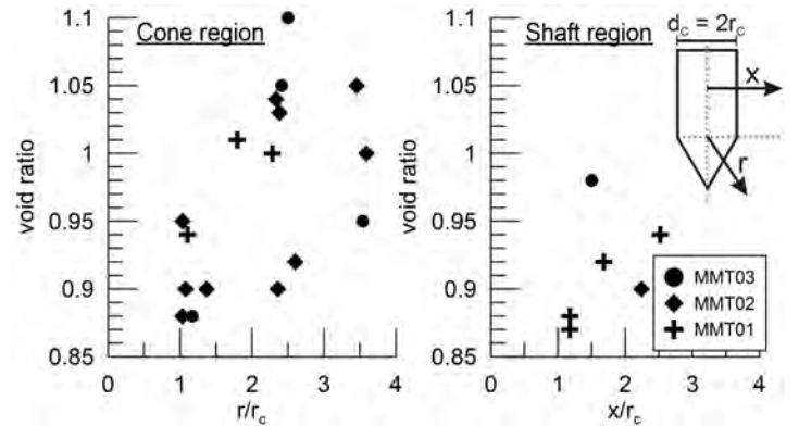
Figure 4. Variation of void ratio values with the normalized distance either r/r_c or x/r_c in the different specimens.
