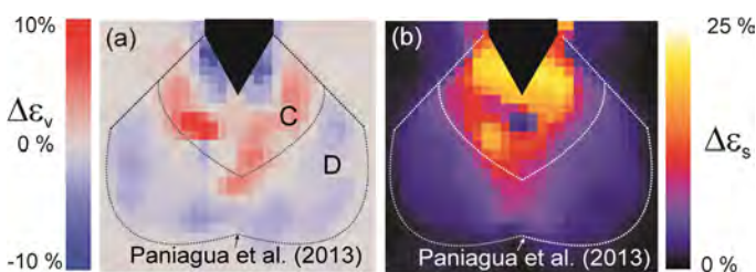
Figure 1. (a) Incremental volumetric strains and (b) incremental shear strains for a penetration increment of 5 mm (Paniagua et al. 2013). C: compaction and D: dilation.
