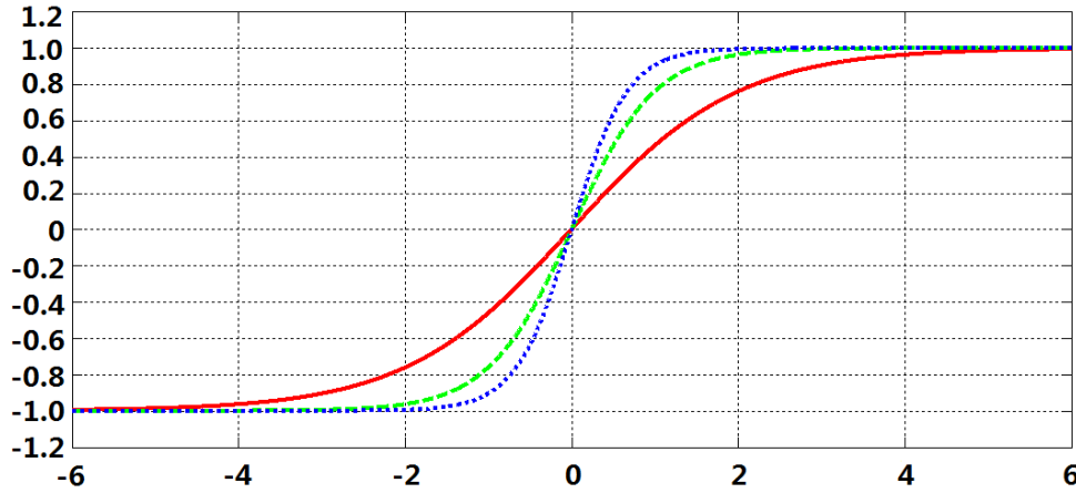
Fig. 4.7 Bipolar Sigmoid function for activation function
