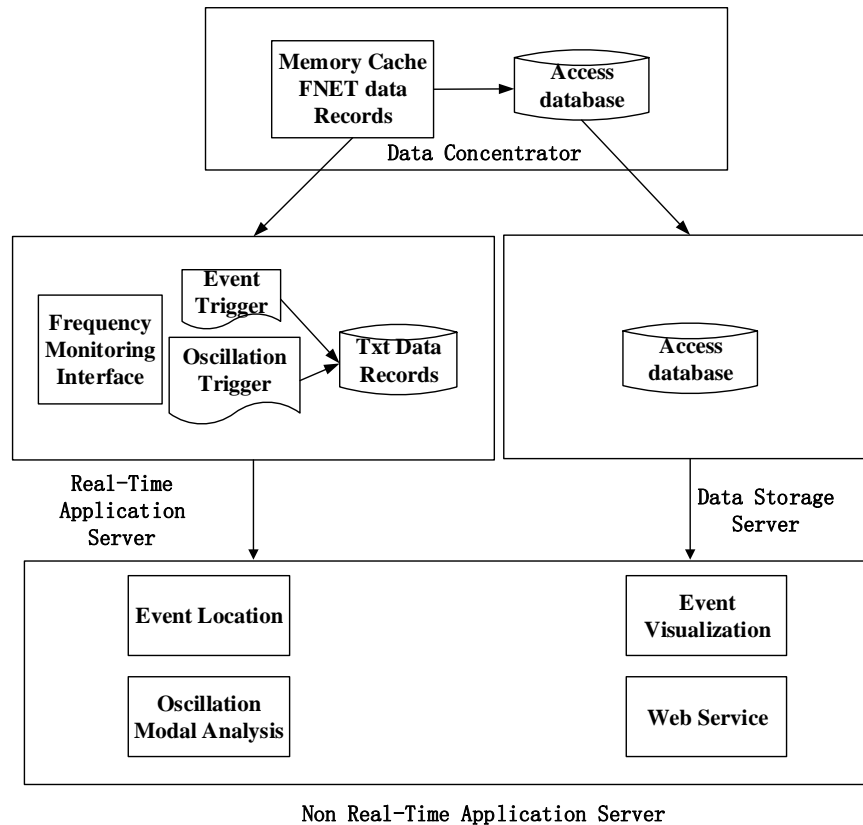
Fig. 3.5 FNET application hierarchy and data flow paths [60]
