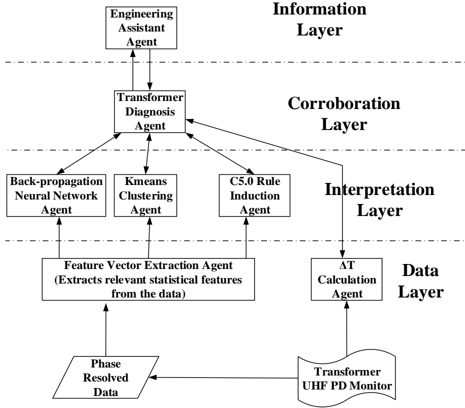
Fig. 3.2 COMMAS architecture [47]
