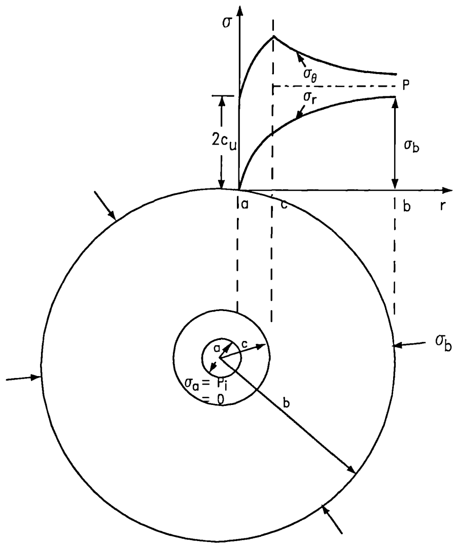
Figure 5.2 Idealized stress distribution for a thick cylinder
